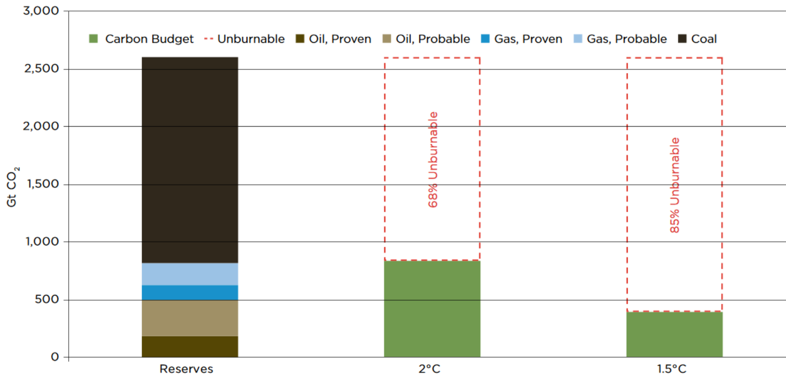
Figure 2: Global Fossil Fuel Reserves Compared to Carbon Budgets for Likely Chance of 2°C and Medium Chance of 1.5°C 2B
